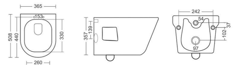
WALL HUNG CLOSET RIMLESS L508, W365, H357MM
