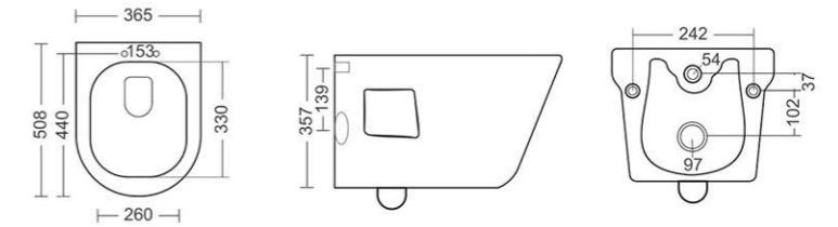
WALL HUNG CLOSET RIMLESS L508, W365, H357MM
