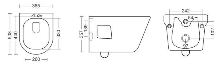
WALL HUNG CLOSET RIMLESS L508, W365, H357MM
